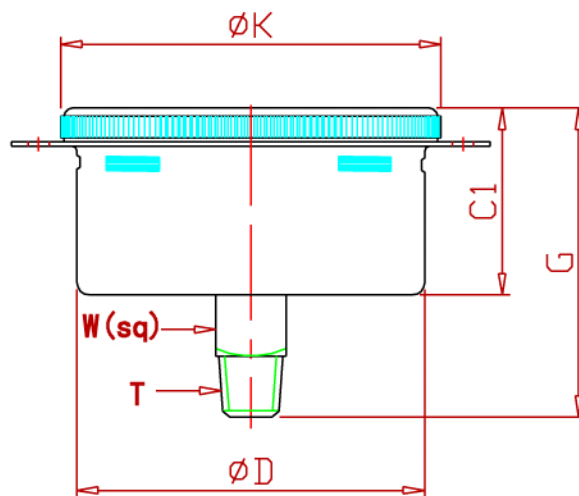
FRONT FLANGE (CBM/FF) (313 Type)
